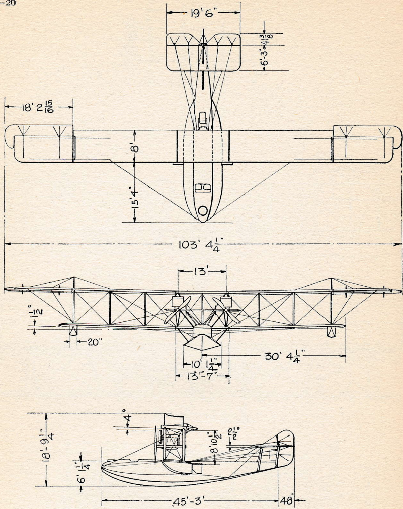
NAVAL AIRCRAFT BUREAU OF CONSTRUCTION AND REPAIR MODEL "F.5-L" 1918-2 LIBERTY 12 330(EACH) H.P. MOTOR 5 90 M.P.H.
