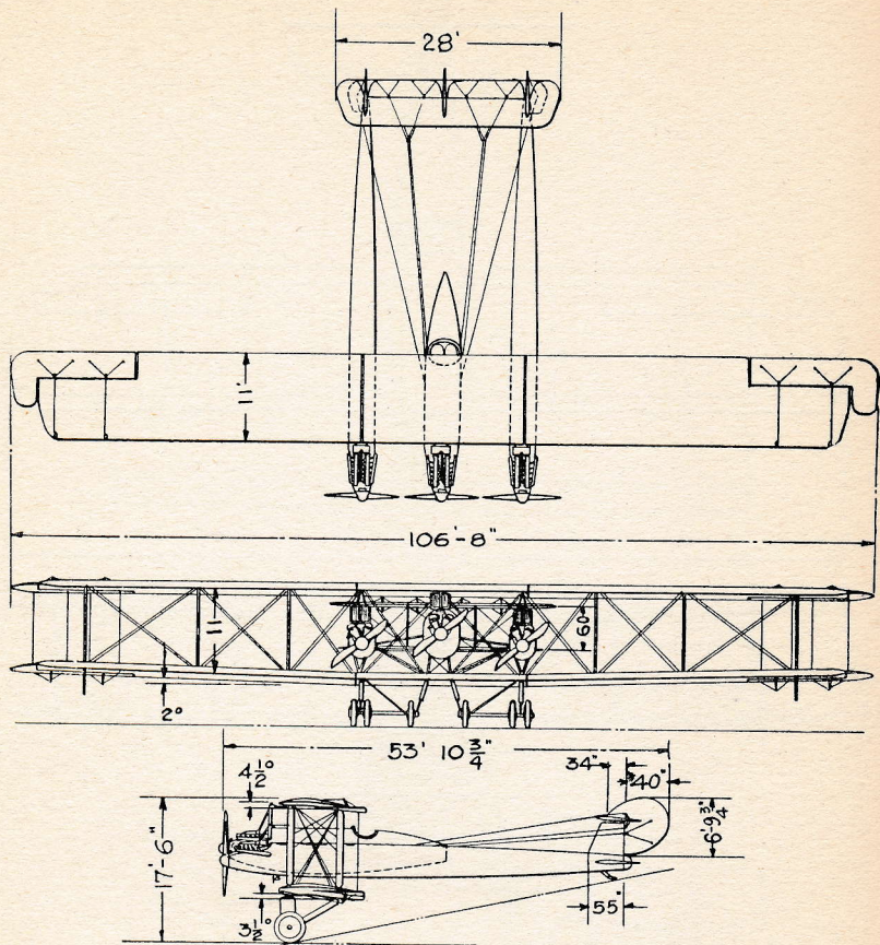
L.W.F. ENGINEERING COMPANY. NEW YORK - COLLEGE POINT L.I.N.Y. MODEL "H" GIANT BOMBER 1920. U.S. AIR SERVICE - 3-400 H.P. (EACH) LIBERTY MOTORS 110 M.P.H.
