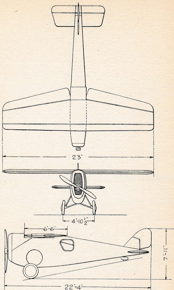
DAYTON WRIGHT COMPANY DAYTON OHIO MODEL "RB" MONOPLANE-1920 GORDON BENNETT ENTRY- HALL SCOTT & CYL. 240 H.P. MOTOR APPROX. SPEED 195 M.P.H.
