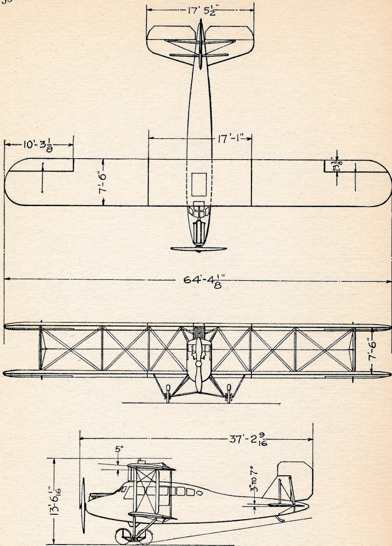
THE CURTISS AEROPLANE AND MOTOR CORPORATION GARDEN CITY L.I.N.Y. CURTISS 10 PASSENGER "EAGLE" 1920-CURTISS "C-12" OR "LIBERTY 12" MOTOR-400 H.P.-100 M.P.H.
