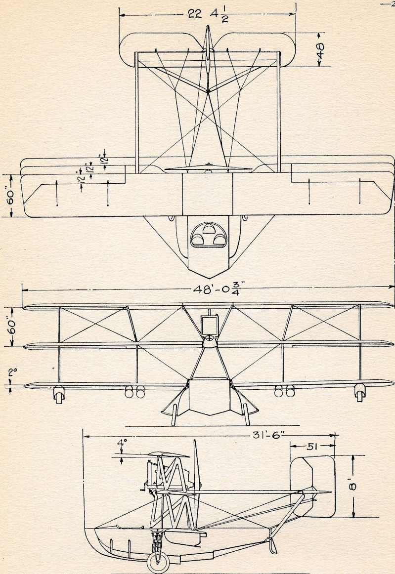
SPERRY AIRCRAFT CORPORATION FARMINGDALE , L.I. N.Y. "AMPHIBIAN" OCT. 1918-LIBERTY 12 CYL. MOTOR-370 H.P.85M.P.H.
