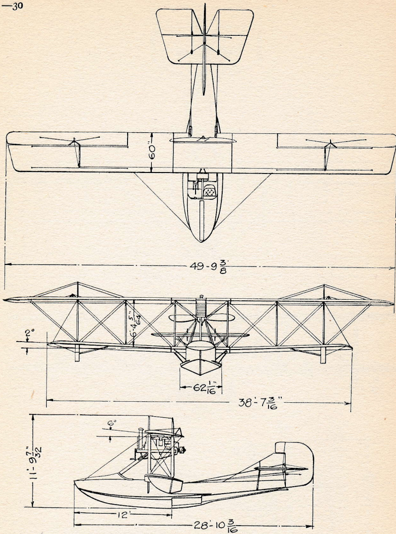
THE CURTISS AEROPLANE AND MOTOR CORPORATION GARDEN CTY L.I.N.Y. CURTISS "SEAGULL" 1919-CURTISS "G6" 150 H.P. MOTOR 76 M.P.H.
