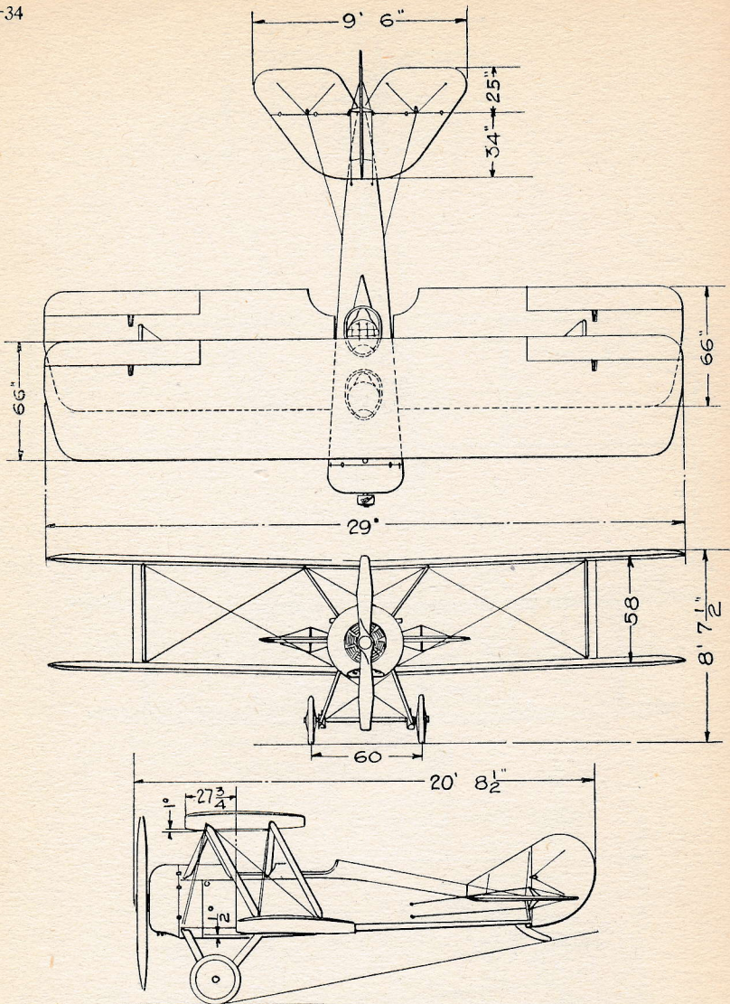
THOMAS-MORSE AIRCRAFT CORPORATION ITHACA, N.Y. MODEL "S-6" FEB. 1919 - LE RHONE 80 H.P. ROTARY MOTOR 105 M.P.H.
