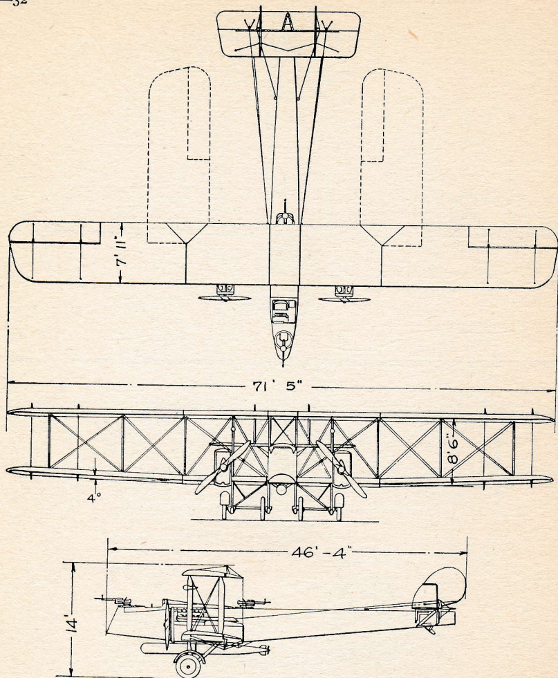
THE GLENN L. MARTIN COMPANY CLEVELAND, OHIO. MODEL "M.T." TORPEDO PLANE 1919-2 LIBERTY 400 H.P. (EACH) MOTORS 114 M.P.H
